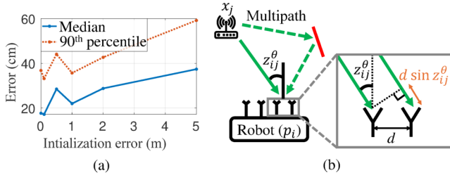
Figure 3: (a) Impact of AP initialization errors: APs have been initialized at varying errors up to 5 m compared to ground truth. The median and 90 th percentile errors have been plotted. The optimizer fails to converge above 5 m of error. (b) Wi-Fi bearings ( \theta ) measured using a linear antenna array with antenna separation d . The additional distance d \sin(\theta) traveled by the signals can be exploited to estimate the bearing
