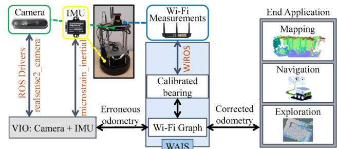
Figure 1: Visual inertial odometry measurements, corrupted by motion drift, are input into WAIS’s module. Combining these measurements with Wi-Fi measurements from WiROS provides online corrected odometry measurements 2 . Lidar Inertial odometry or wheel odometry can also be used.
